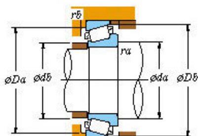
Hm218248/10 Bearing 2D drawings and 3D CAD models
